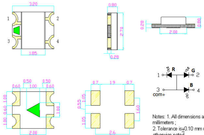
Recommended Soldering Pad
